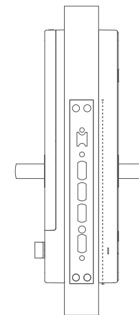
Measuring the length of the front plate
